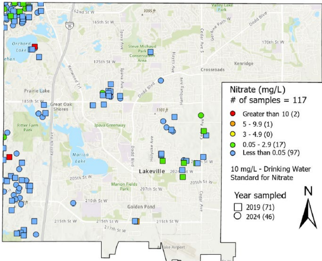
Figure 3. Nitrate results in untreated water from outside spigot
